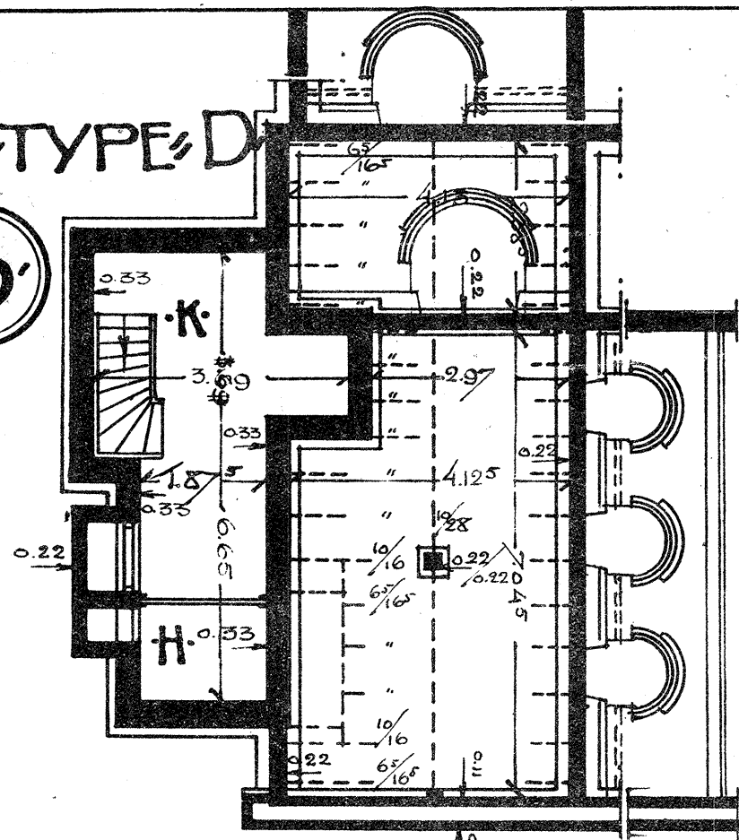
FUNDEERING
